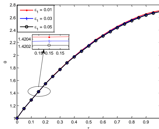
Fig. 3. Effect of \varepsilon_1 on the temperature profile.
