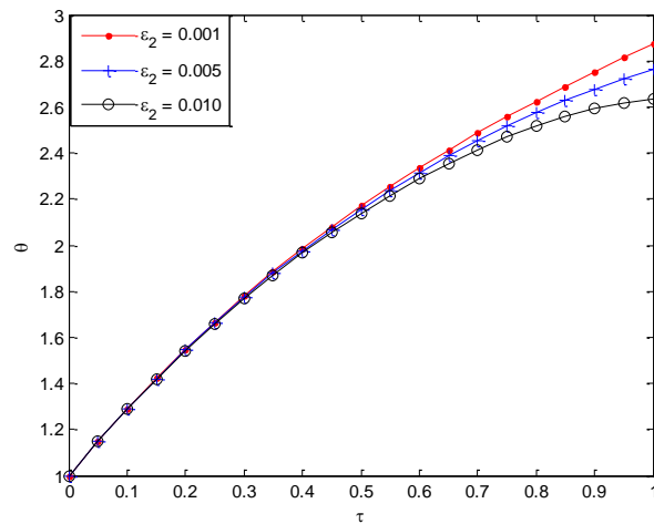
Fig. 4. Effect of \epsilon_2 on the temperature profile.
