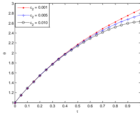
Fig. 4. Effect of \epsilon_2 on the temperature profile.
