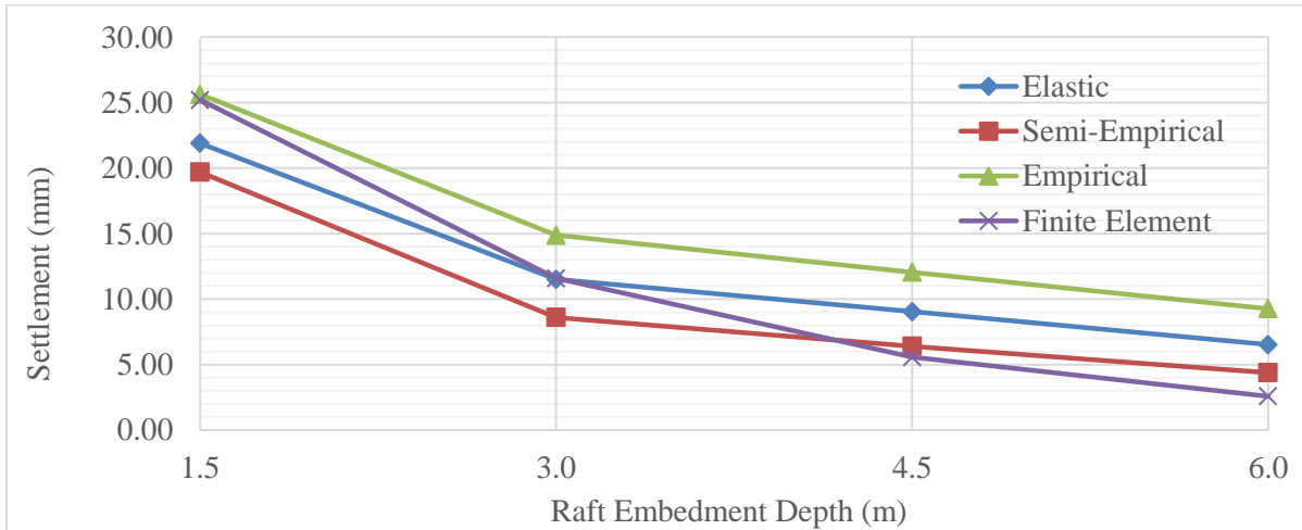
Fig. 5. Settlement versus embedment depth for 100 kN/m 2 applied pressure.
