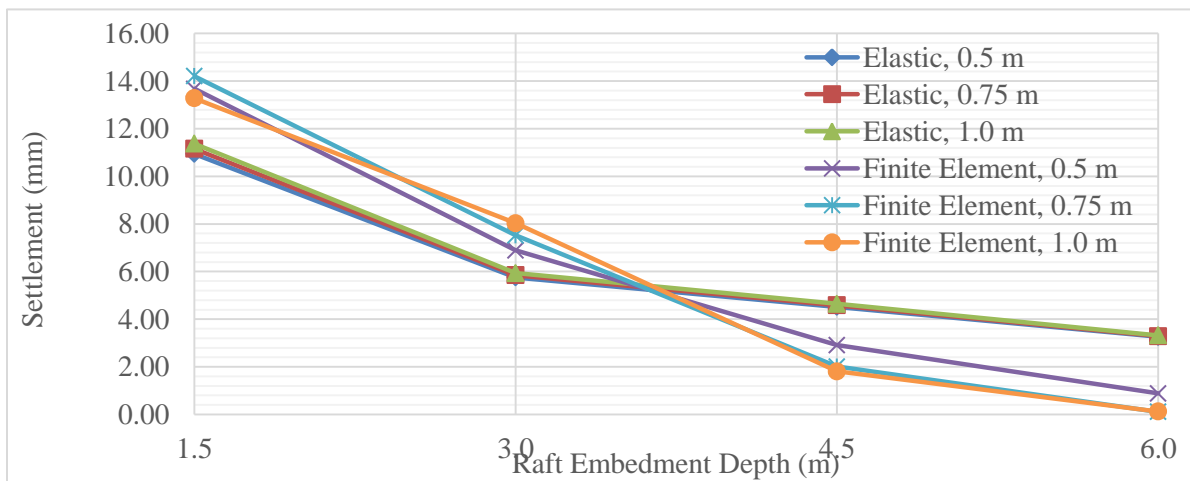
Fig. 10. Settlement versus depth showing the effect of raft thickness for 50 kN/m 2 .
