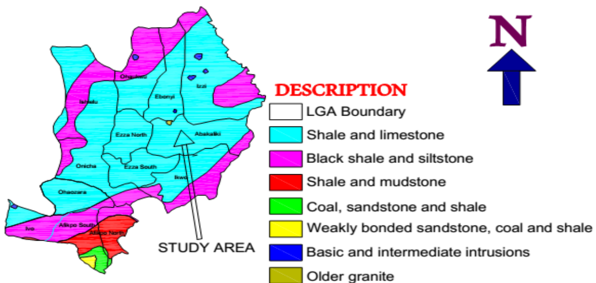
Fig. 1. Geological map of Ebonyi State is showing the soil groups.
