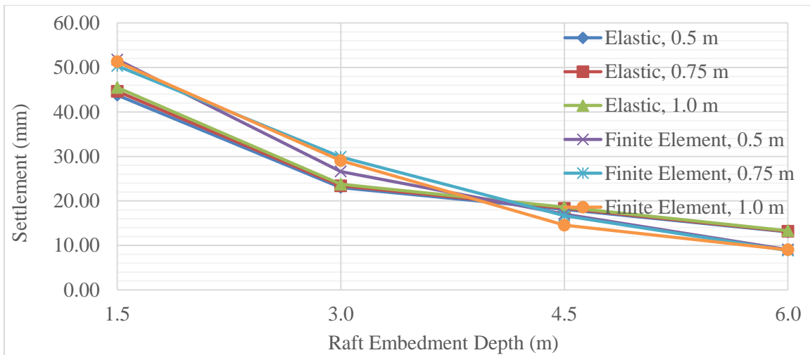
Fig. 12. Settlement versus depth showing the effect of raft thickness for 200 kN/m 2 .
