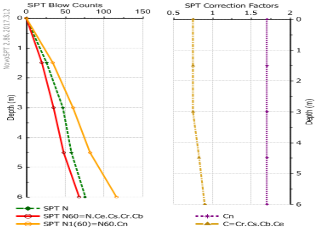
Fig. 2. Soil boring log layering and SPT results.
