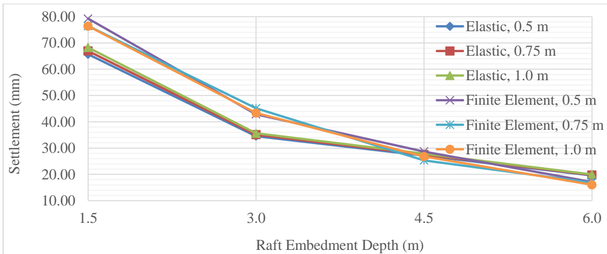
Fig. 13. Settlement versus depth showing the effect of raft thickness for 300 kN/m 2 .
