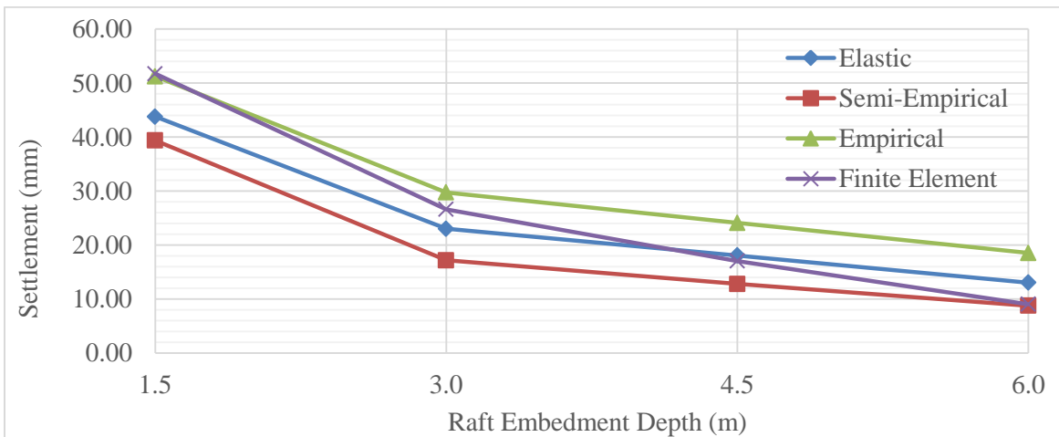
Fig. 6. Settlement versus embedment depth for 200 kN/m 2 applied pressure.
