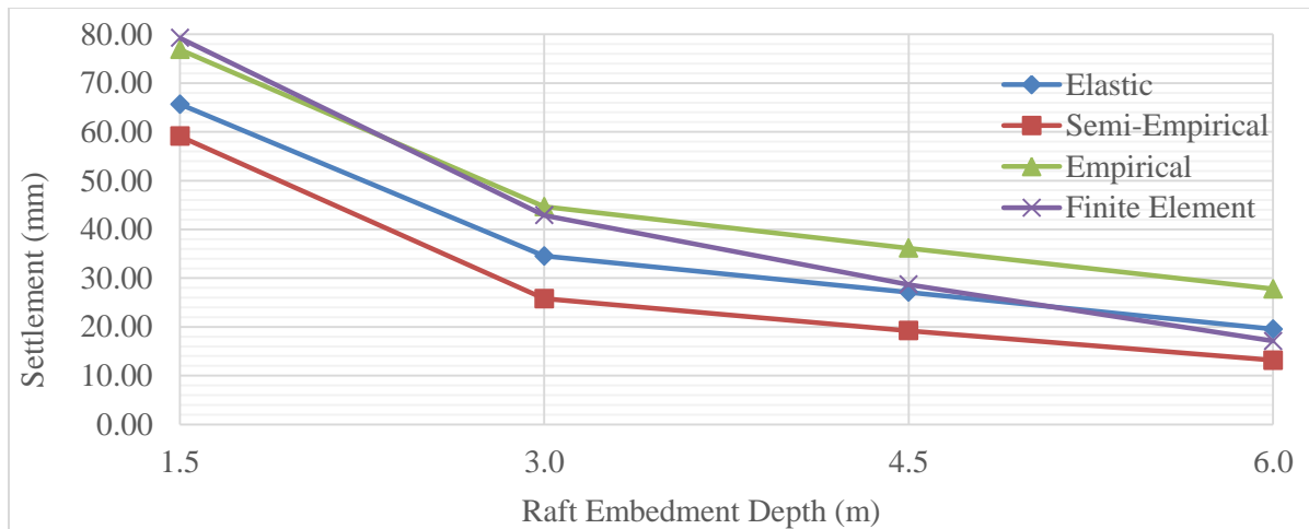
Fig. 7. Settlement versus embedment depth for 300 kN/m 2 applied pressure.
