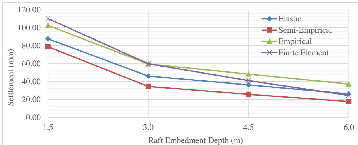
Fig. 8. Settlement versus embedment depth for 400 kN/m 2 applied pressure.
