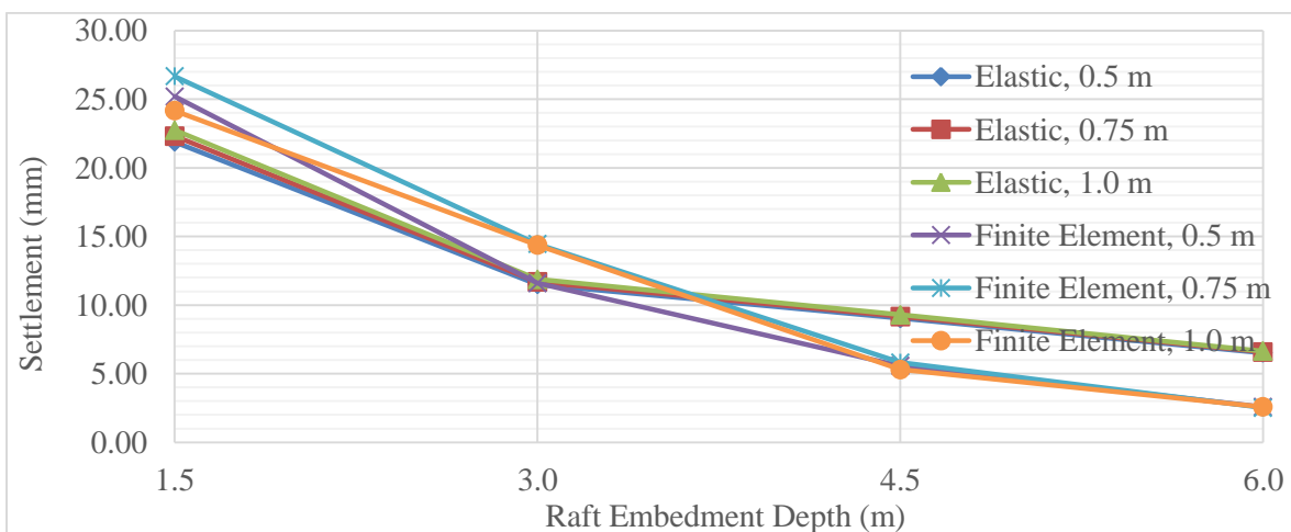
Fig. 11. Settlement versus depth showing the effect of raft thickness for 100 kN/m 2 .
