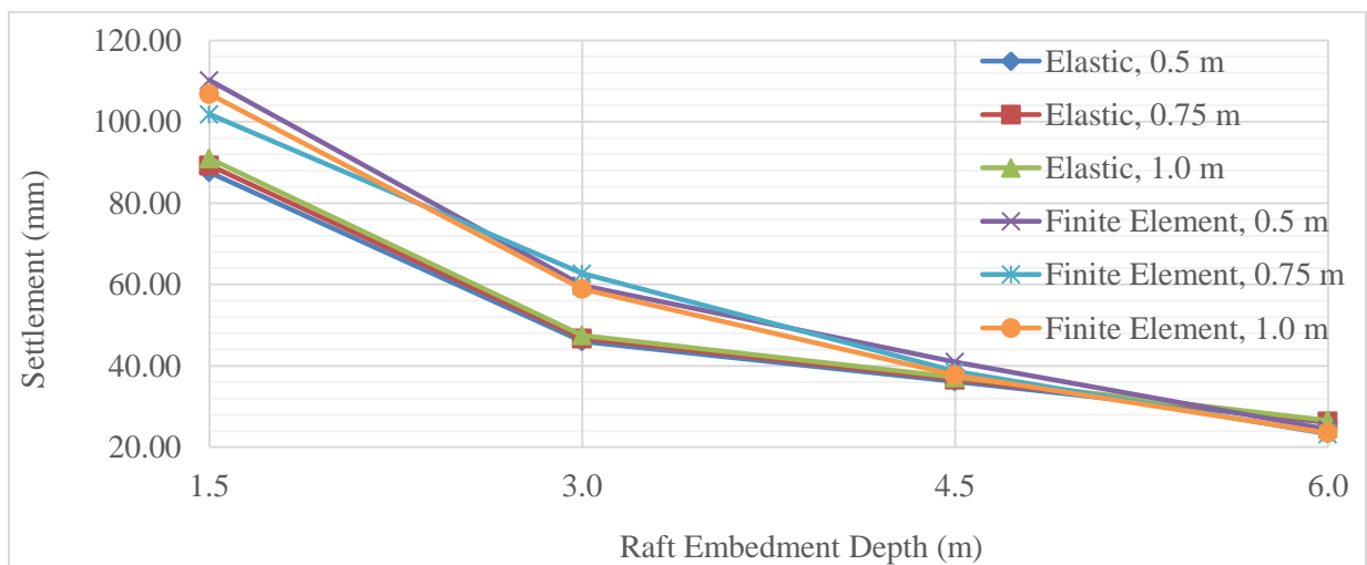
Fig. 14. Settlement versus depth showing the effect of raft thickness for 400 kN/m 2 .
