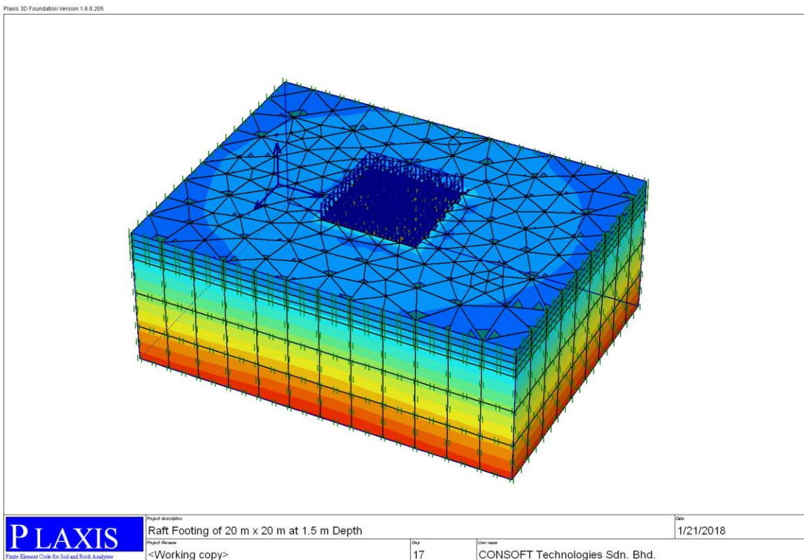
Fig. 3. 3D soil model used for numerical analysis.
