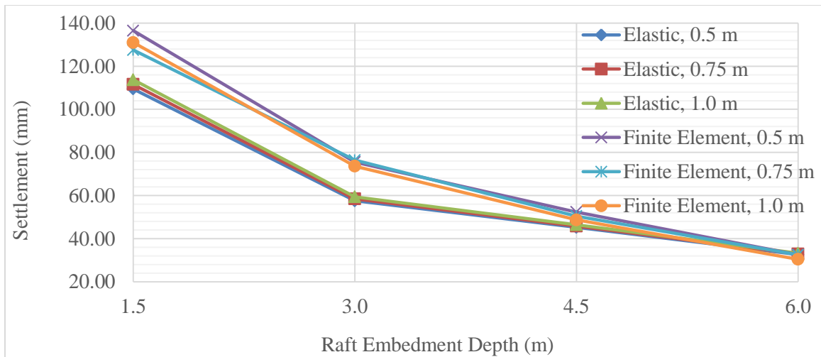
Fig. 15. Settlement versus depth showing the effect of raft thickness for 500 kN/m 2 .
