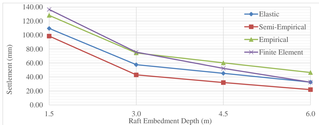
Fig. 9. Settlement versus embedment depth for 500 kN/m 2 applied pressure.
