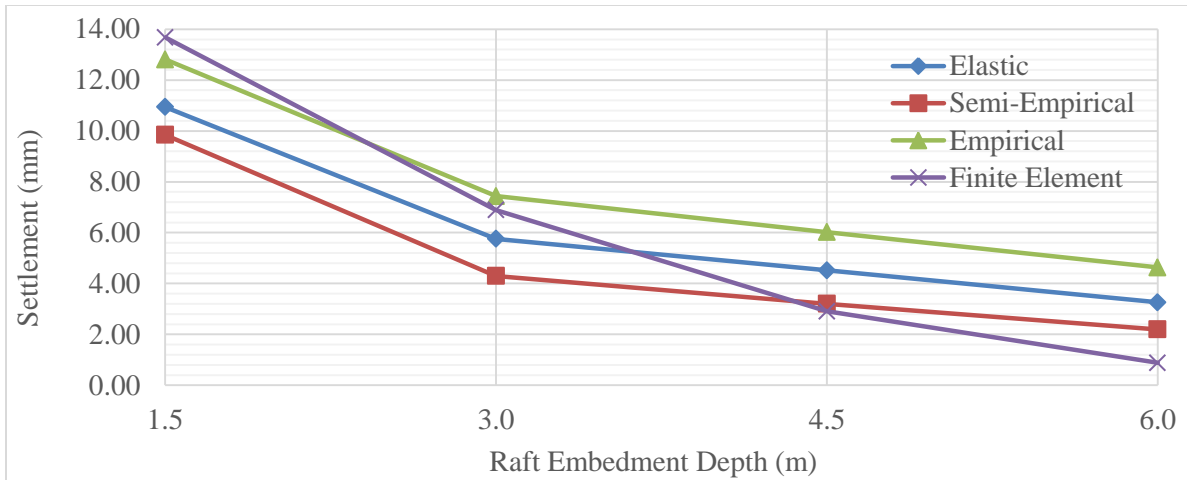
Fig. 4. Settlement versus embedment depth for 50 kN/m 2 applied pressure.
