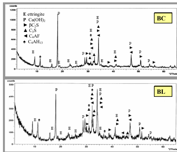
Fig. 8. Radiogram of concrete specimens after 365 days of curing.
