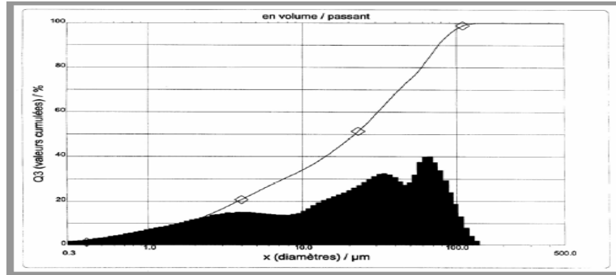
Fig. 2. Particle size distribution of the slag.
