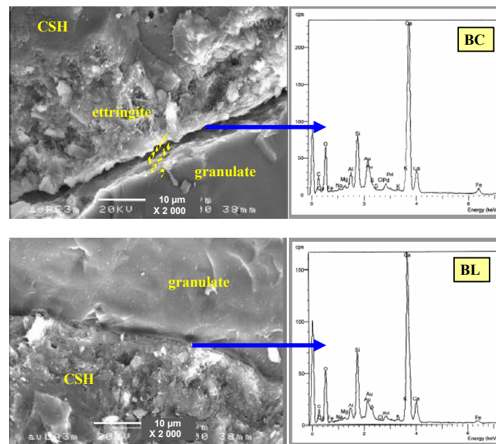
Fig. 10. SEM observation of transition halo of different concretes after 365 days of curing.
