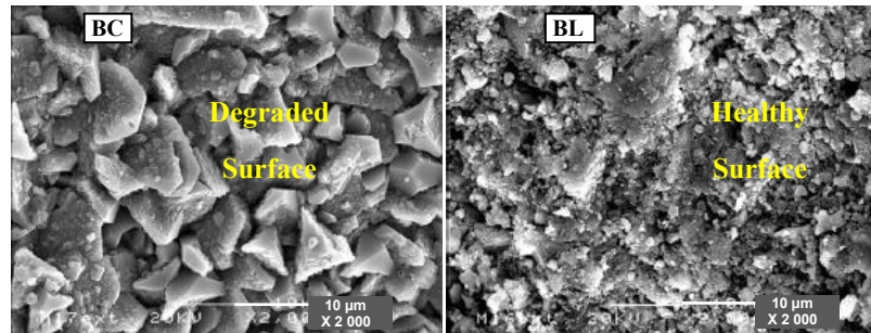
Fig. 5. SEM observation of the surface of concrete specimens after 365 days of curing.
