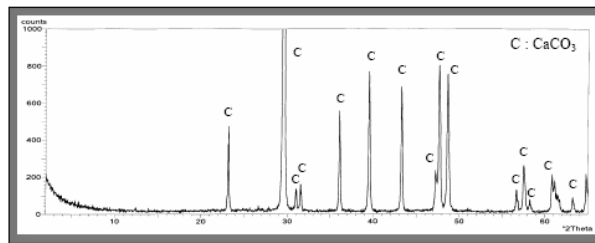
Fig. 6. Radiogram of the calcite observed on the surface of various concretes.
