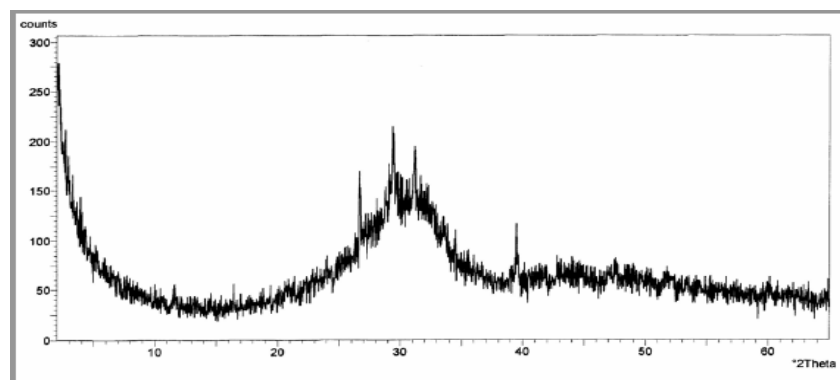
Fig. 1. Diffractogram of the slag.
