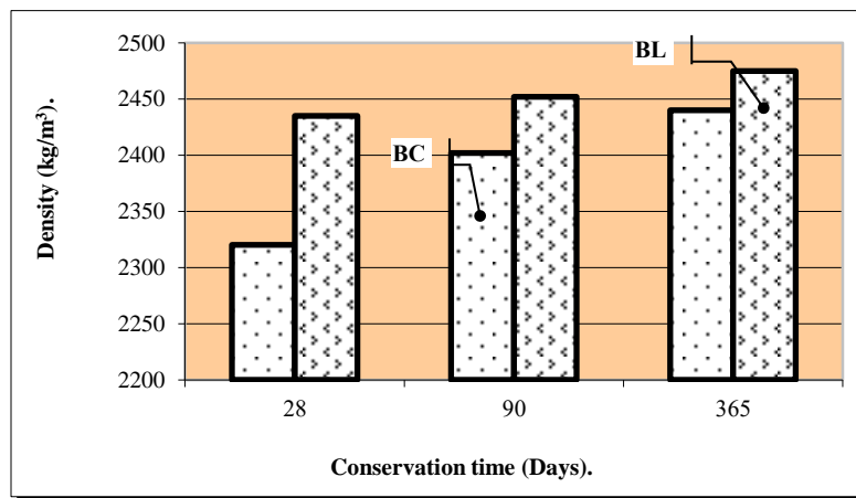
Fig. 3. Evolution of the concretes density as a function of curing time.
