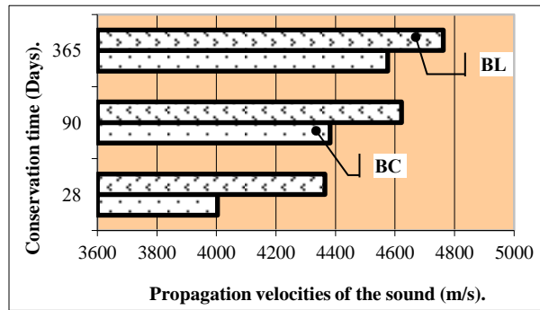
Fig. 9. Evolution of sound propagation velocities through concrete specimens as a function of curing time.
