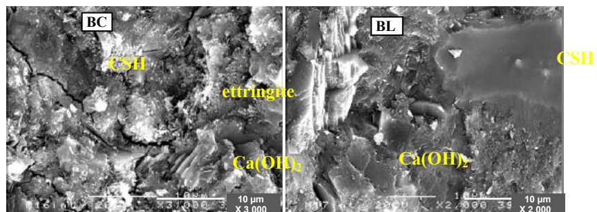
Fig. 7. SEM observation of the internal micro-structure of concrete specimens after 365 days of curing.
