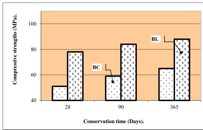
Fig. 4. Evolution of compressive strength as a function of curing time.
