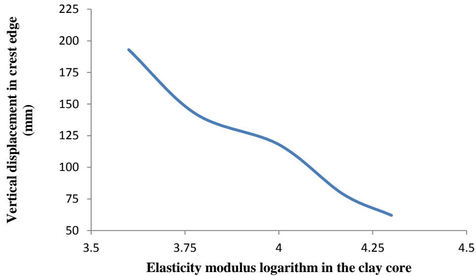
Fig.4. Changes diagram of vertical displacement in crest edge (mm).
