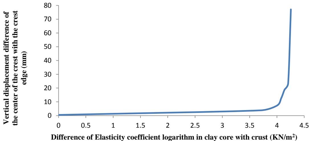
Fig.3. Changes diagram of the vertical displacement difference of the center and crests edge.
