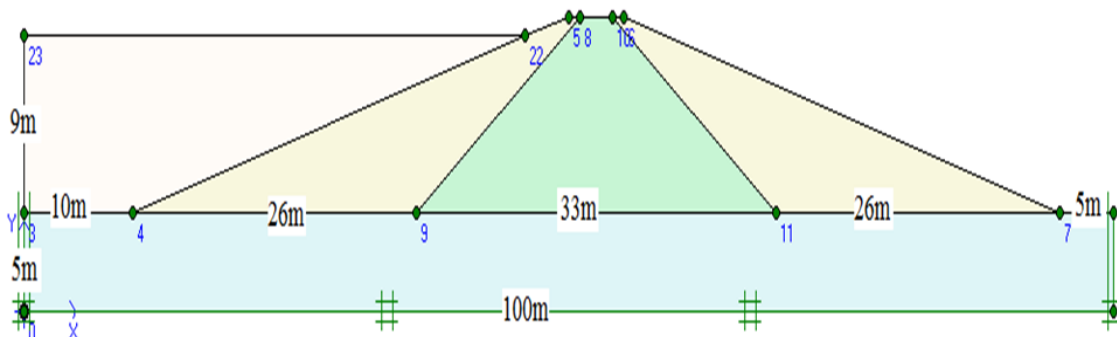
Fig. 1. Geometry of the numerical model.
